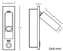
Cutout size: L160 x W40 x H60mm
