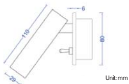
Cutout size: D50 x H50mm
