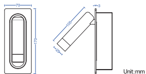
Cutout size: L150 x W55 x H45mm
