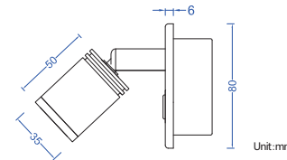
Cutout size: D50 x H50mm
