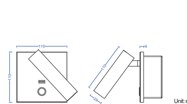
Cutout size: L95 x W60 x H45mm
